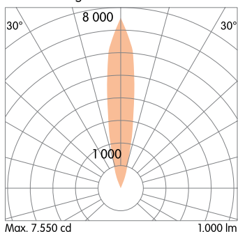
10° Beam Angle
