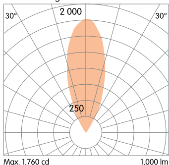
50° Beam Angle
